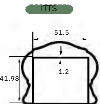
Aluminum for Gate post 2"x3.5"
