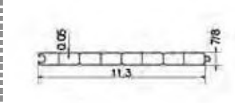
7/8"×1.3"T&G (3 Gap)
