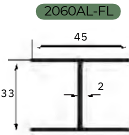
Aluminum stiffener for ribA luminumstiffenerfor rail, 1.75 x 5.5" Flat Slot Rail 2"x6"
