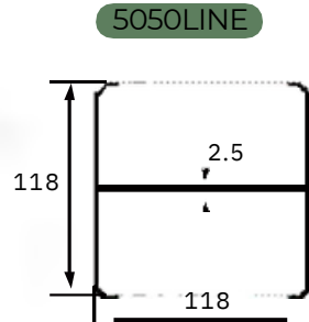
Aluminum mounting for Line Post 5"x5"
