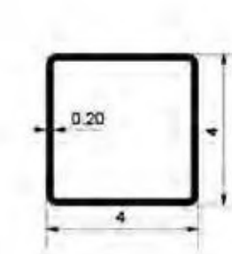
4040P20 4"×4"Post
