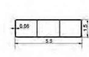
1555RR 1.5"×5.5"Rib Rail
