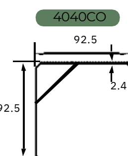
Aluminum mounting for Corner Post 4"x4"
