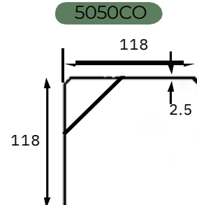
Aluminum mounting for Corner Post 5"x5"
