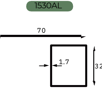
Aluminum stiffener for Rail 1.5"x3.5"
