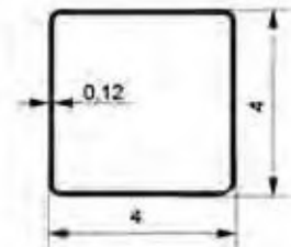
4040P12 4"×4"Post
