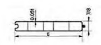
7/8"×6"T&G Panel
