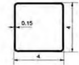
4040P15 4"×4"Post
