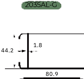
Aluminum for Gate post 2"x3.5"
