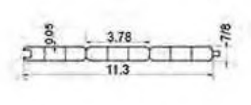
7/8"×1.3"T&G (2 Gap)
