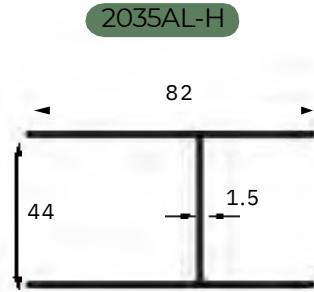
Aluminum stiffener for Hollow Rail 2"x3.5" and T-Rail
