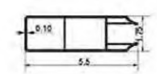
1-3/4"×5-1/2"Slot Rail
