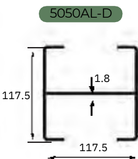
Aluminum stiffener for Post 5"x5"
