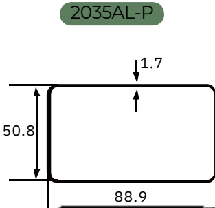
Aluminum Pipe 2"x3.5"
