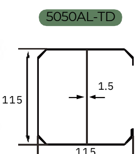
Aluminum stiffener for Post 5"x5"x0.2" Thick
