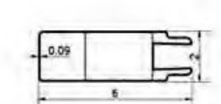
2060SR2 2"×6"Slot Rail
