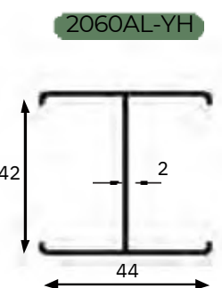
Aluminum stiffener for Rib Rail 2"x3.5" and Slot Rail 2"x6"
