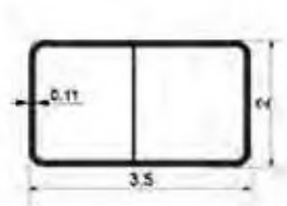
2035RR 2"×3-1/2"Rib Rail
