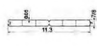
7/8"×1.3"T&G (1 Gap)
