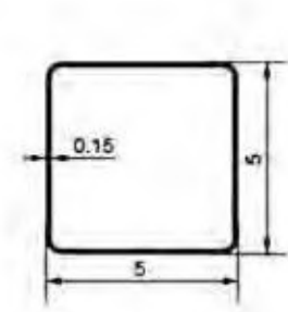
5050P15 5"×5"Post
