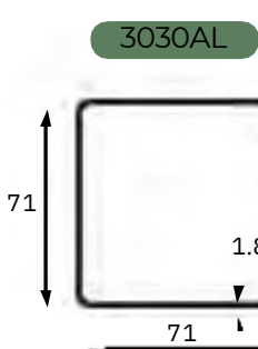
Aluminum stiffener for Post 3"x3"
