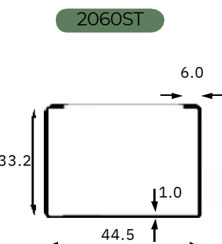
Aluminum for Gate Rail 1.5"x5.5"
