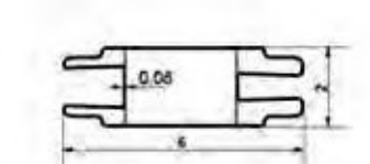
2"×6"Double Slot Rail
