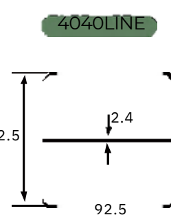
Aluminum mounting for Line Post 4"x4"
