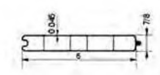
7/8"×6"T&G Panel
