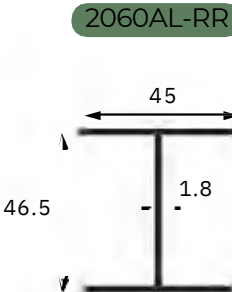
Aluminum stiffener for Rail 2"x6"
