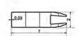
2070SR 2"×7"Slot Rail
