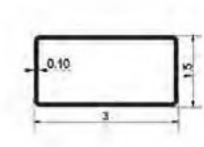
1530HR 1.5"×3"Hollow RAIL
