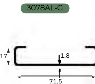
Aluminum stiffener for Picket 7/8"x3"
