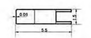
1-1/2"×5-1/2"Slot Rail
