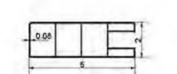
2060SR3 2"×6"Slot Rail
