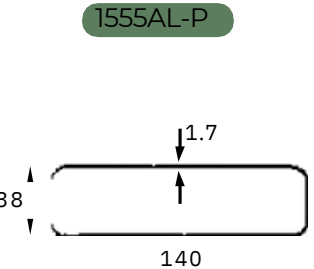
Aluminum mounting for Corner Post 5"x5"
