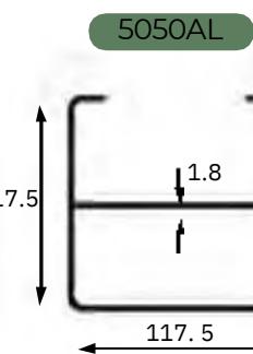
Aluminum stiffener for Post 5"x5"
