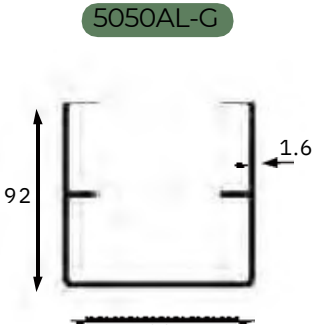
Aluminum stiffener for Gate Post
